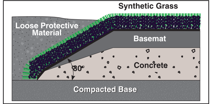
Loose-Fill with Concrete
