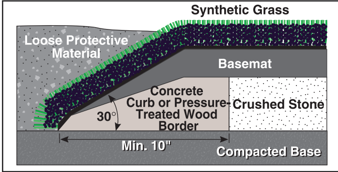
Loose-Fill with Crushed Stone (contained)
