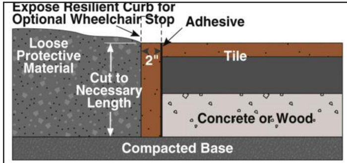
Loose-Fill – Resilient Rubber Curb
