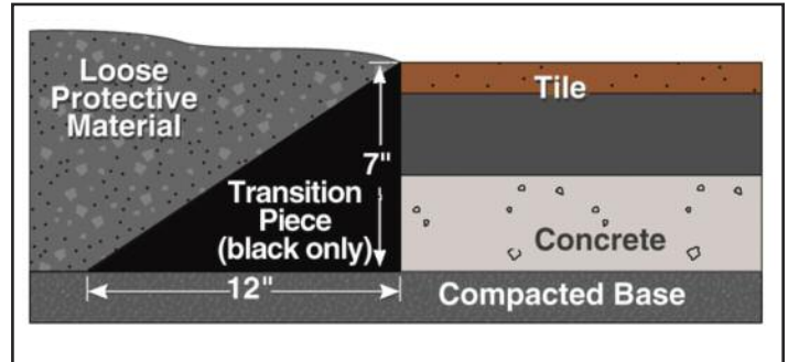
Loose-Fill – Resilient Transition Piece Edge
